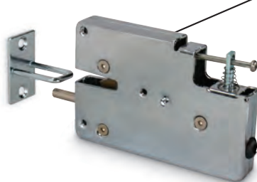
Electronic Lock with Spring Pin (for Standard Lockers)
